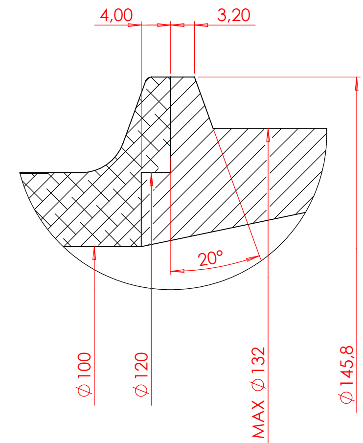
Detail B
